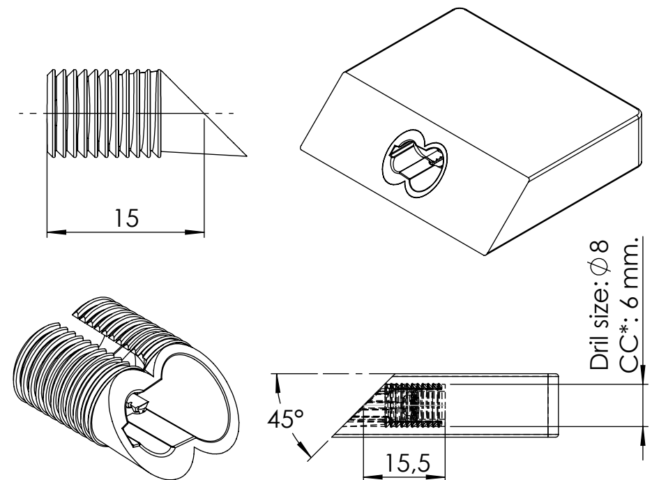
Fixi 45° Keyhole installation guide:
